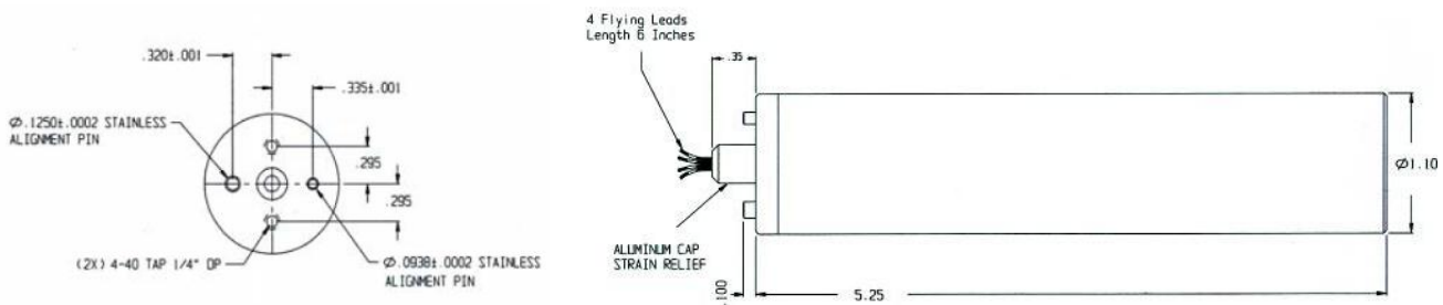
CHS110TB Dimensions
