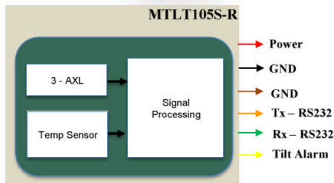
Platform Leveling
